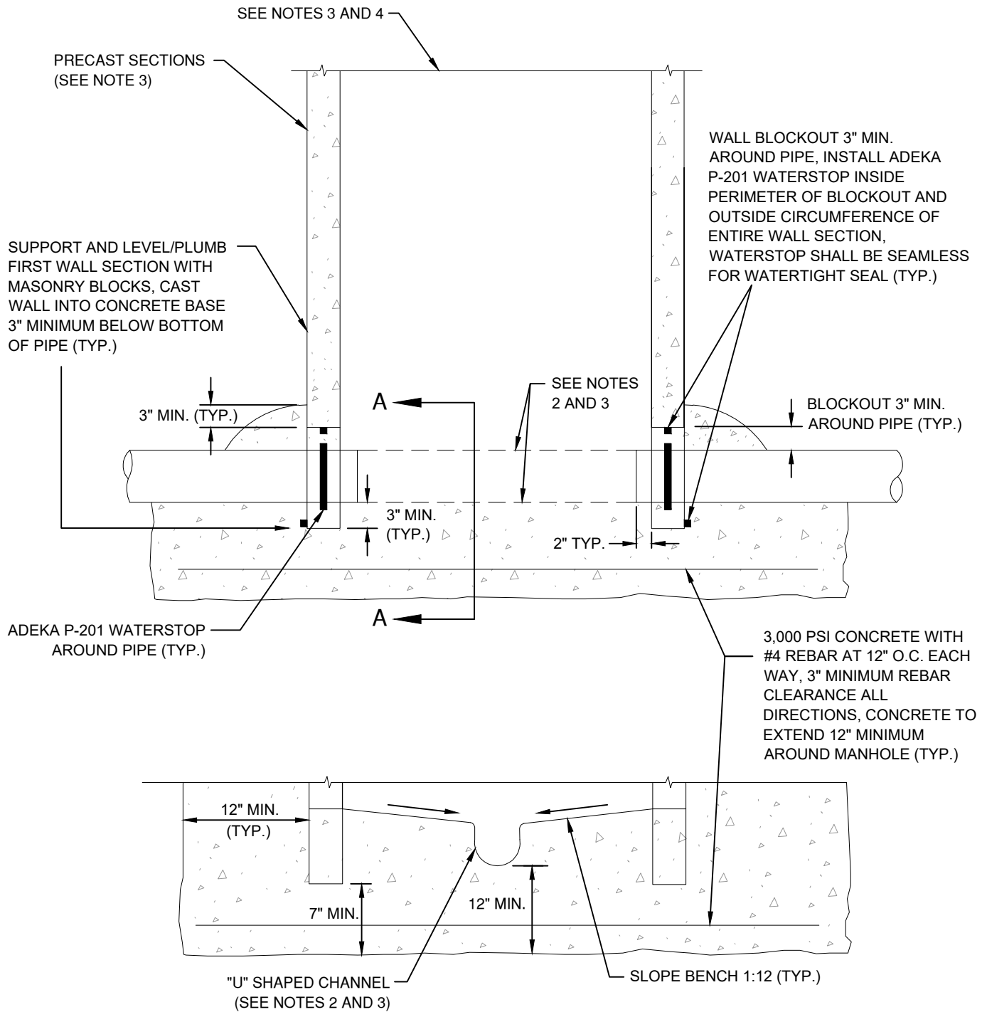
SECTION "A-A"
